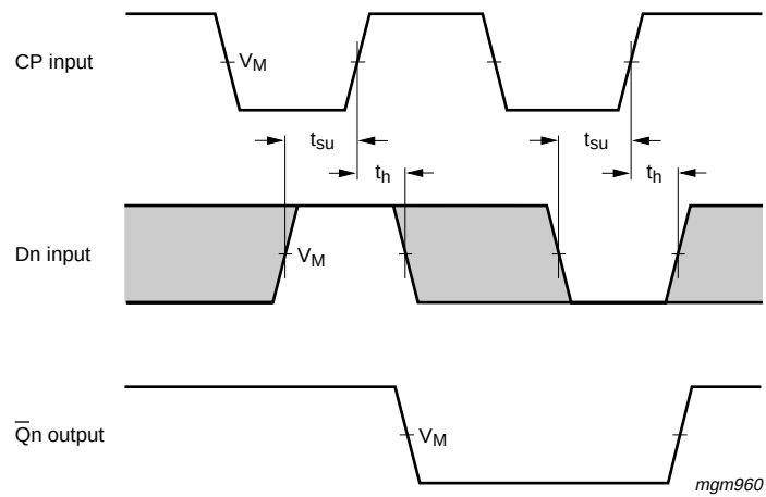
Fig 8. Waveforms showing the data set-up and hold times for Dn input.
